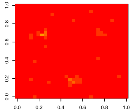
Figure 5: Posterior group regression coefficient image
